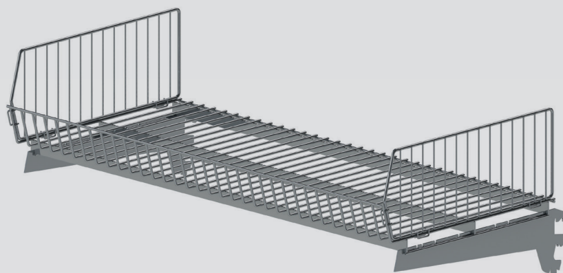
WIRE RACK – HOOKS ITSELF TO THE FITTING MECHANISM OF THE CANTILEVER GONDOLA WHITE ZINC FINISH
